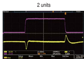
2 units IT6006D-500-40 Setting: voltage 100V current 56A Load current: 60A
