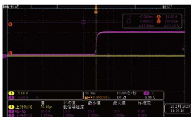
Single unit
