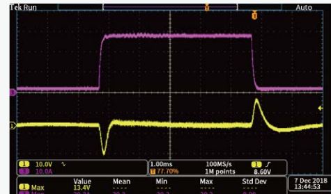
Paralleled units
