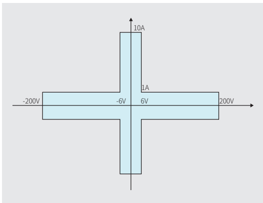
IT2806 200V output characteristic curve (pulse only)
