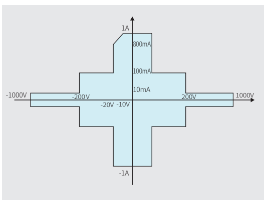
IT2801 1000V output characteristic curve
