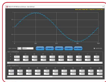
Loading 50 order harmonic components
