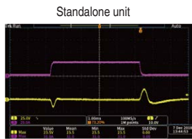
Standalone unit IT6006D-500-40 500V/40A/6kW Setting: voltage 100V current 28A Load current: 30A
