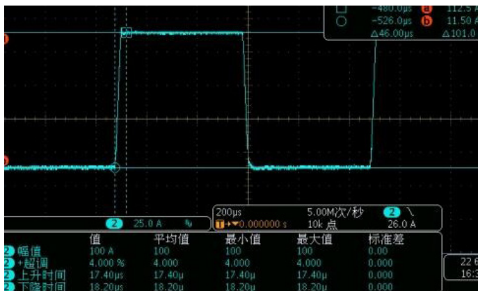
IT8733P+ (80V,120A,600W) 10A~110A dynamic waveform (current slope 5A/ \mu\text{s} )
