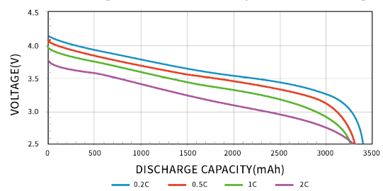
discharge characteristics(by rate of discharge)
