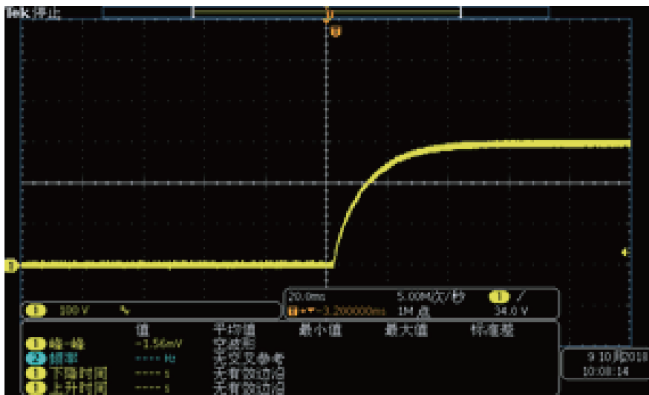
Start-up inrush current over current range, high-speed build-up voltage electric CV Priority
