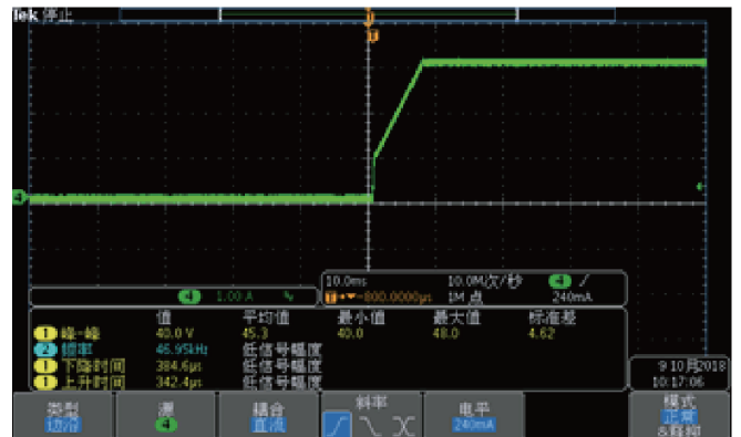
Seamless battery charging and discharging at high speed with no overshoot switching CC Priority
