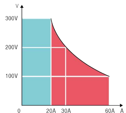
+ ITECH Operating range Operating range of other 300V products on the market
