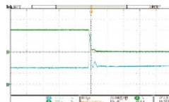
No soft stop function, voltage overshoot
