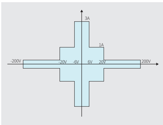
IT2806 200V output characteristic curve (DC or pulse)
