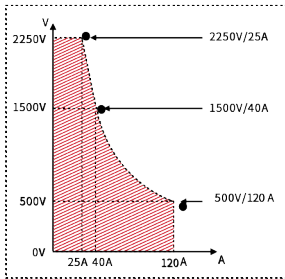
CP curve of IT6000D
