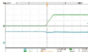
IT8906A-1200-240 rated power 6kW withstand transient 8kW loading
